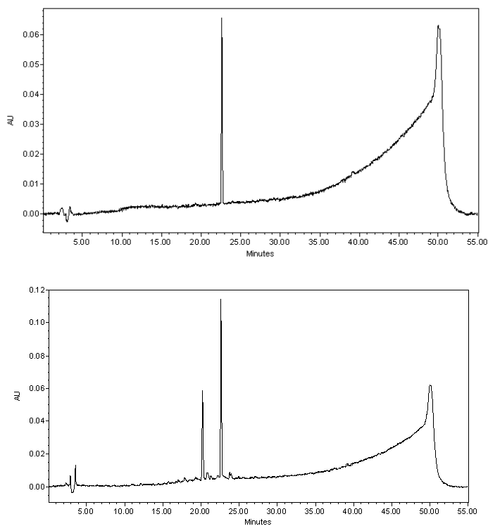
Figure 3. HPLC chromatogram of nodularin in standard solution (A) and extract (B).
